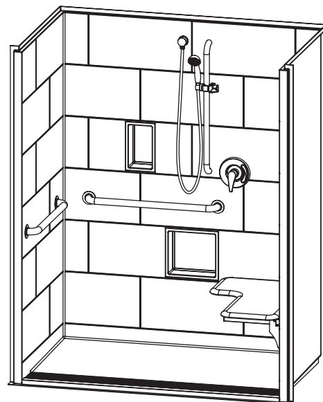
Right hand configuration shown with optional soap dish
