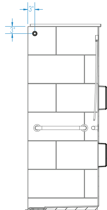
SECTION C-C
