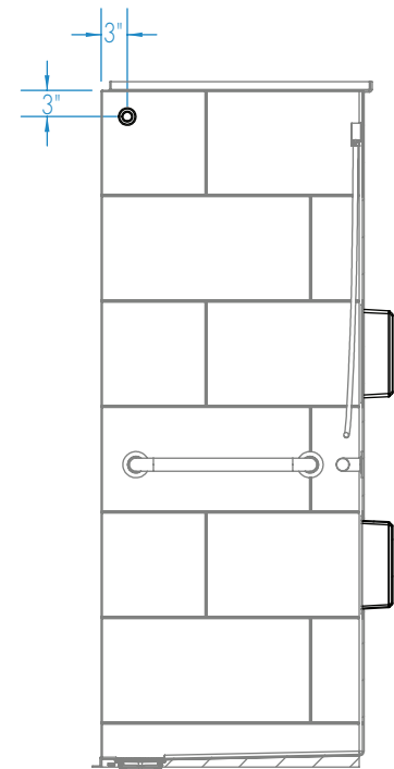
SECTION C-C
