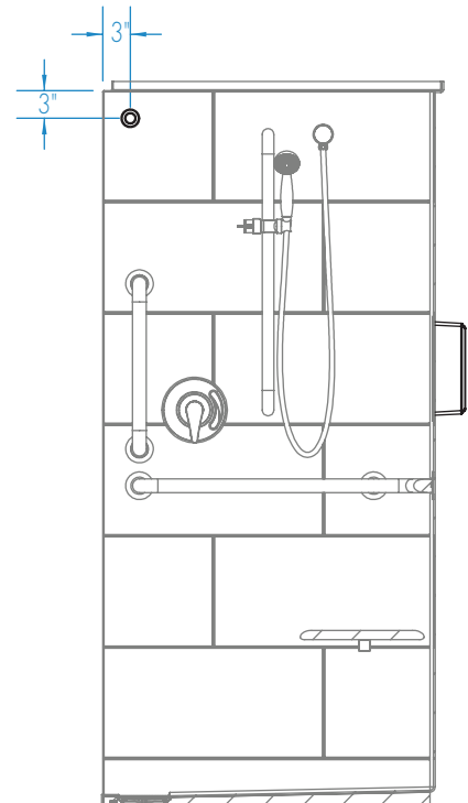
SECTION C-C
